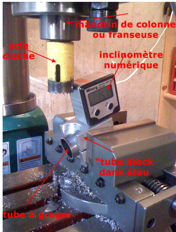
grugeage colonne_tube block.jpg
